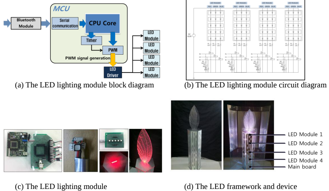
Fig. 12. The LED lighting device structure
