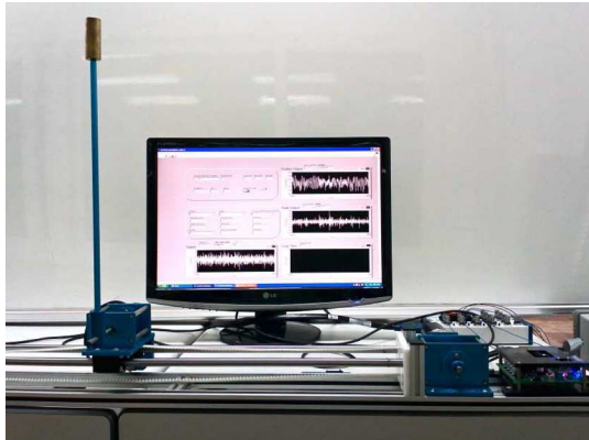
Fig. 10. Linear inverted pendulum used in the testbed.
