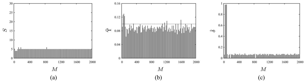
Fig. 5. Number of selected paths \hat{Y} and \hat{\delta} of the basic algorithm with the exponential RTT distribution when \tau_c = 2 ms and \epsilon = 0.1 . (a) The number of selected paths with respect to the sample size. (b) \hat{Y} with respect to the sample size (where the dotted line denotes the given required reliability of \epsilon ). (c) The empirical robustness metric \hat{\delta} with respect to the sample size.
