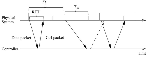
Fig. 2. Timing constraint between the physical system and the controller. The dotted arrow denotes the delivery of a control packet that is abandoned by the physical system because \text{RTT} > \tau_l .
