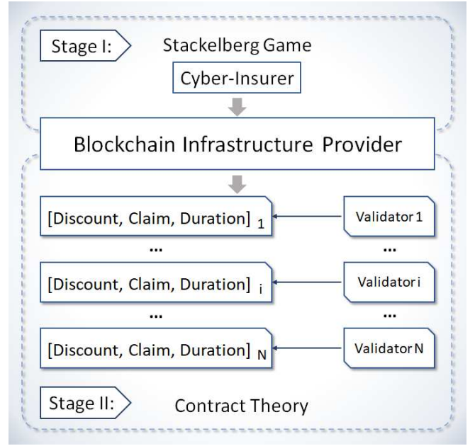
Fig. 3. A two-stage hierarchical game model.
