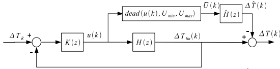
Fig. 3. Resulting feedback-structure when H(z) = \hat{H}(z) .
