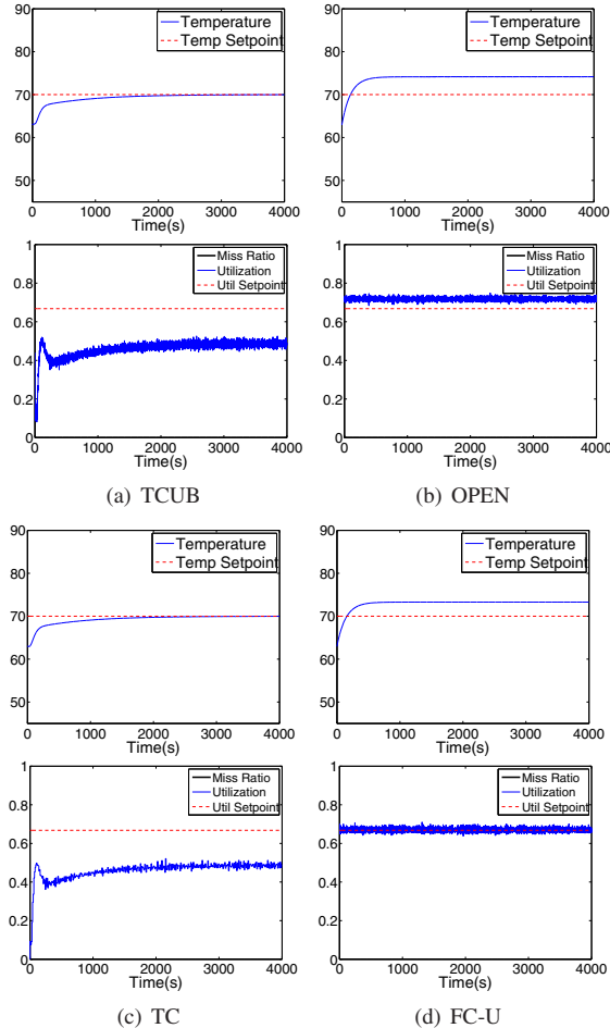
Fig. 9. Performance Comparison with Different Ambient Temperature
