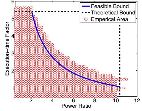
Fig. 7. TCUB Performance with Varying Power Ratio and ETF
