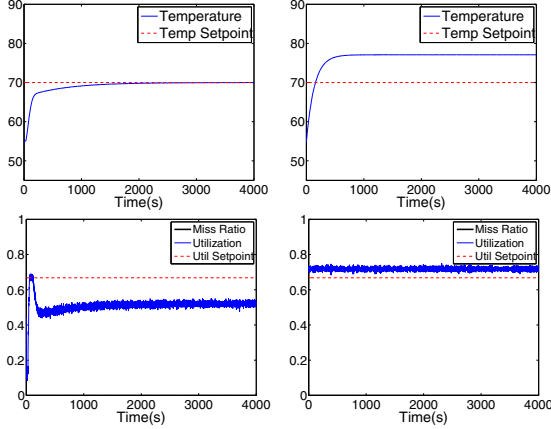
(a) TCUB (b) OPEN (c) TC (d) FC-U Fig. 4. Performance Comparison (Power Ratio = 2)
