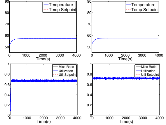
(a) TCUB (b) OPEN (c) TC (d) FC-U Fig. 5. Performance Comparison (Power Ratio = 0.5)
