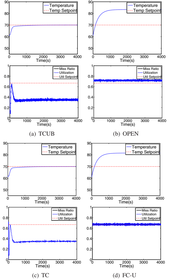
Fig. 8. Performance Comparison with Thermal Fault
