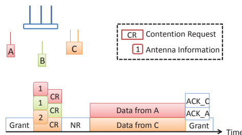
Fig. 4: An illustrative example of communication in CUTS.
