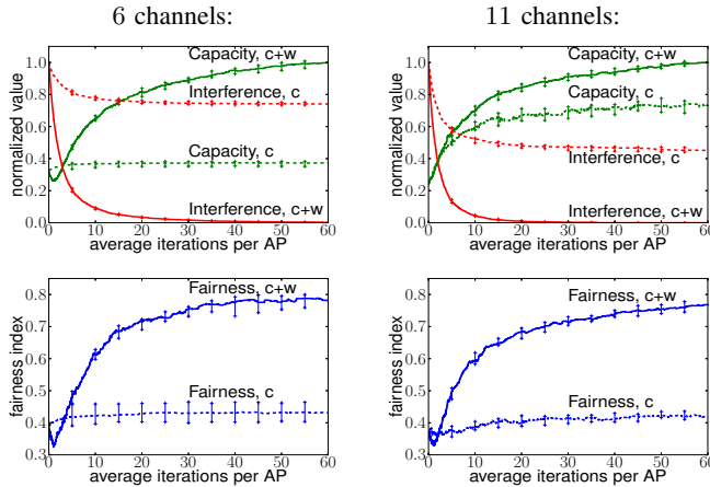
Fig. 4: Capacity, interference and fairness as functions of the number of iterations. We show the values obtained when SAW tunes both the channel center frequency and bandwidth (c+w), and when it tunes only the center frequency (c).
