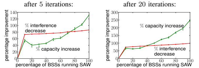
Fig. 5: Percentage of improvement (compared to random allocations of fixed bandwidth channels), as a function of the percentage of BSSs using SAW.
