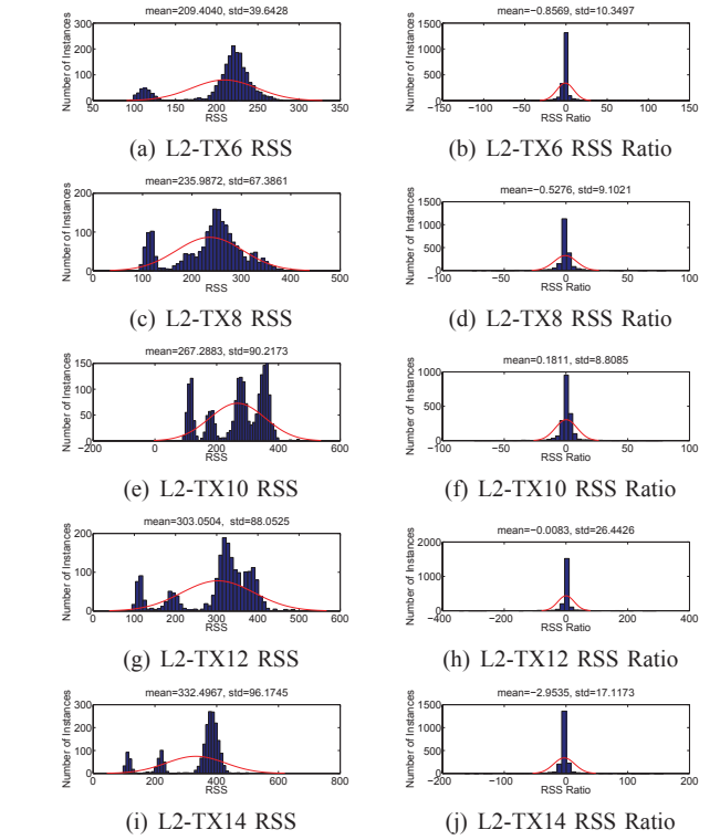
Fig. 4. The measured RSS and RSS-Ratio over transmission powers in the WARP based tests at location L2.
